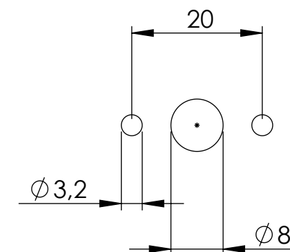
Bohrbild / Hole pattern
