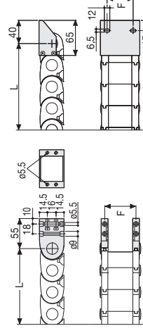
Fig. B Chain fixed outside the radius. (Fig B) See end brackets mounting variations page 31.
