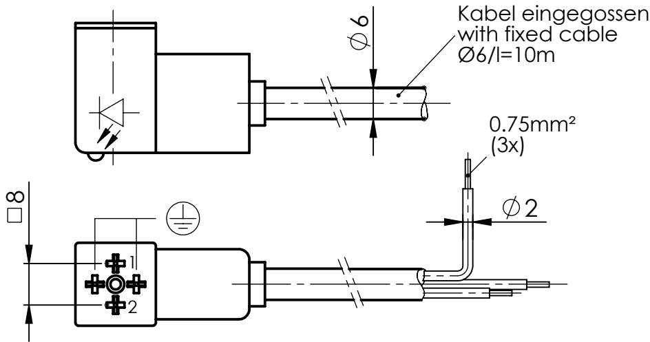
Stecker Pneumatikventile plug pneumatic valve
