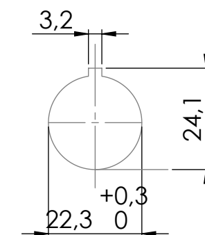
Bohrbild / Hole pattern
