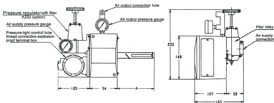
Figure 2 External dimensions
