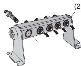
Supply rail with isolation valves for series 551
