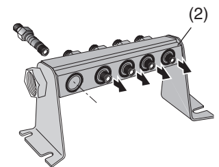
Supply rail with isolation valves for series 551
